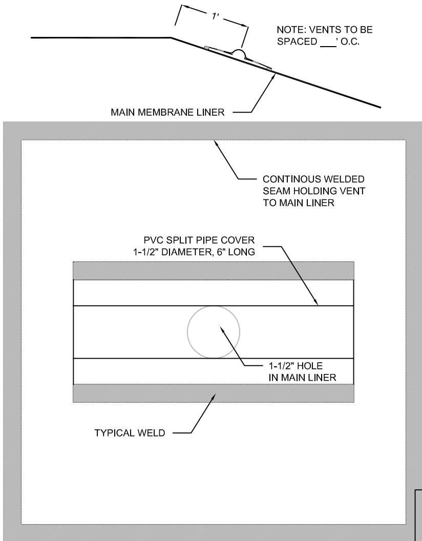
SPLIT PIPE VENT (NTS)
