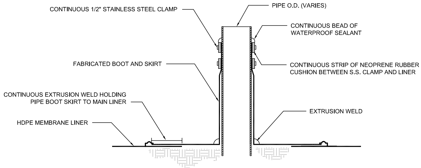
TYPICAL VERTICAL PIPE BOOT DETAIL (NTS)
