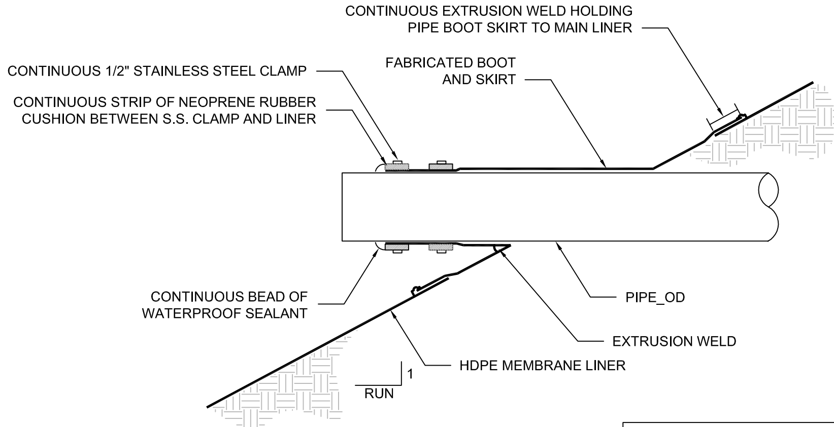
TYPICAL HDPE PIPE BOOT (NTS)
