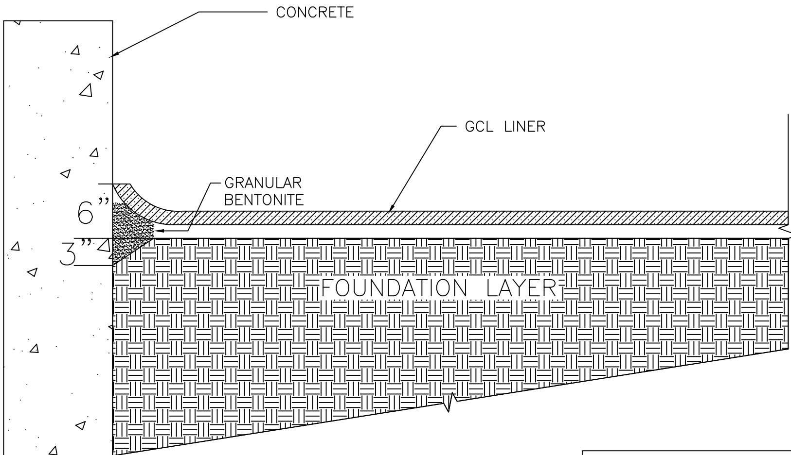
TYPICAL GCL WALL ATTACHMENT
