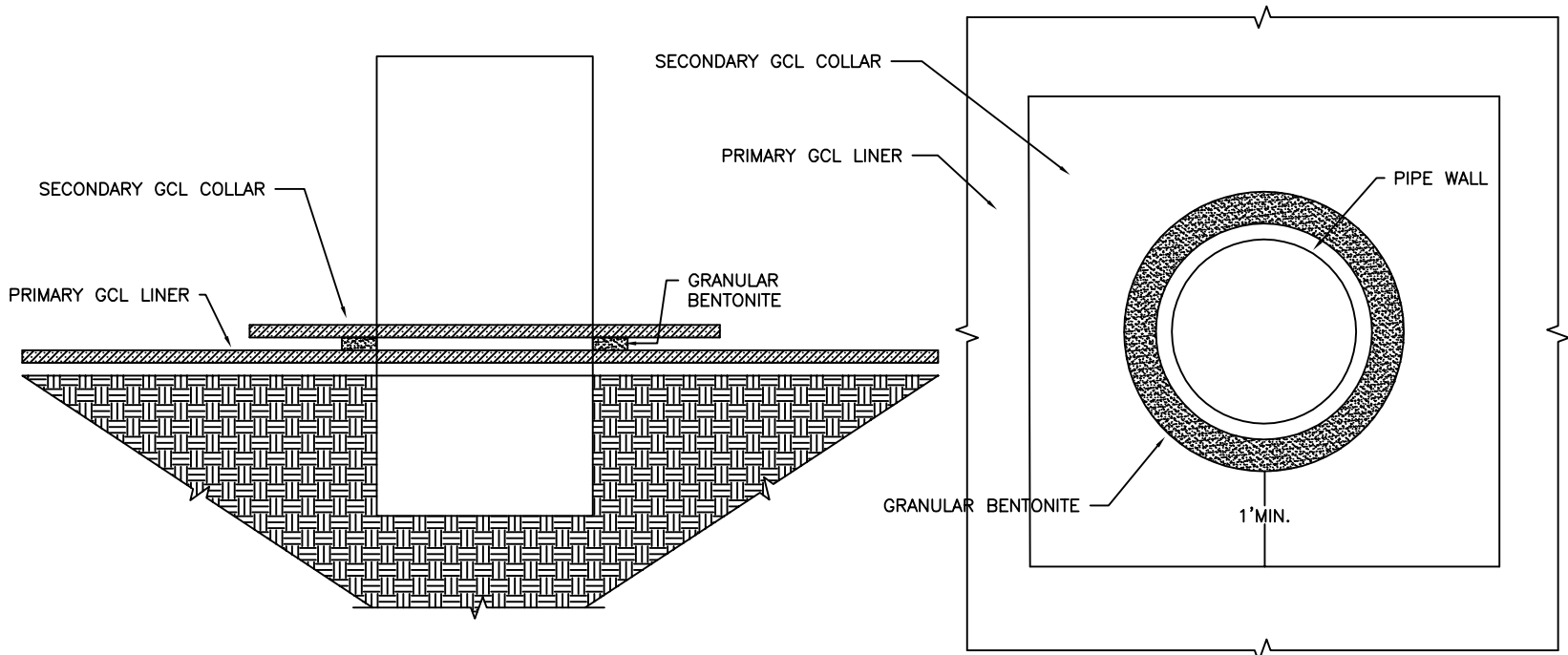
GCL PIPE PENETRATION (90 DEGREES)
