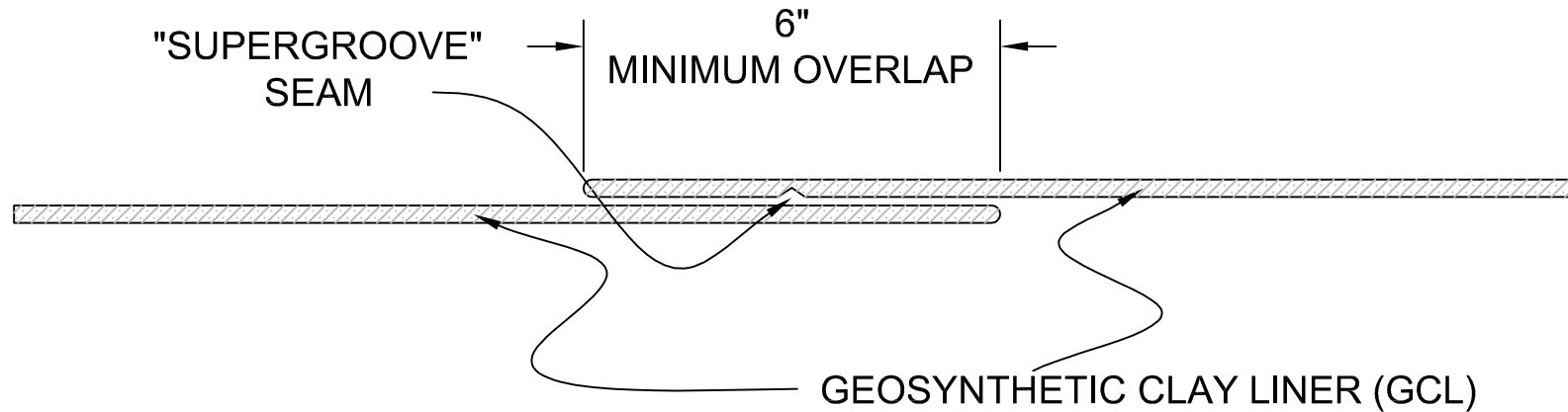
TYPICAL GCL FIELD SEAM WITH "SUPERGROOVE" (NTS)
